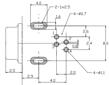
COMPONENT SIDE PCB LAYOUT
